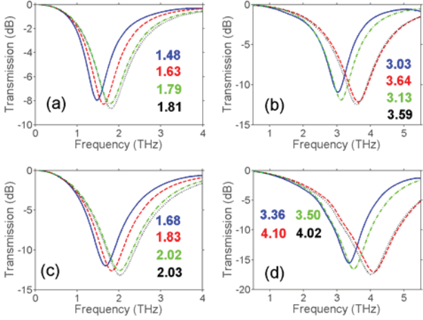
Fig. 2. Spectrums of the co-polarized transmission coefficients (a,c) |\tau_{xx}| and (b,d) |\tau_{yy}| for (a,b) N=1 and (c,d) N=2 , for Faraday (solid blue line), Voigt-Y (dashed red line), Voigt-X (dash-dotted green line) configurations for B_0 = 1 T, and for B_0 = 0 (dotted black line); \epsilon_d = 2.1 . Colored numbers indicate center frequencies of the stopbands in THz.
